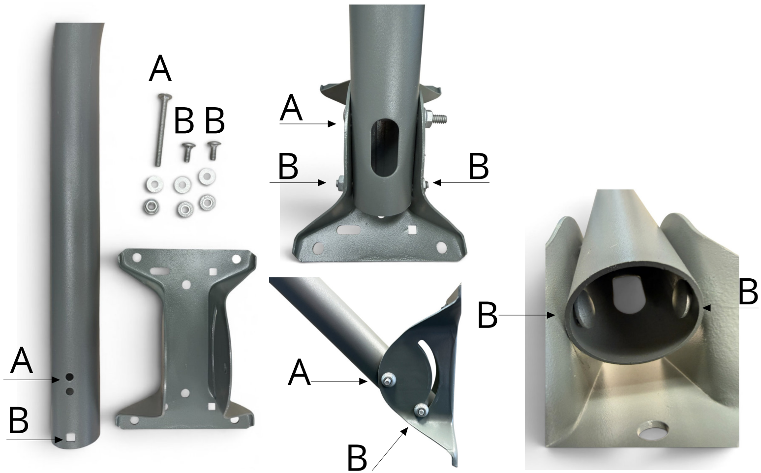
Assemble FOOT Mount
